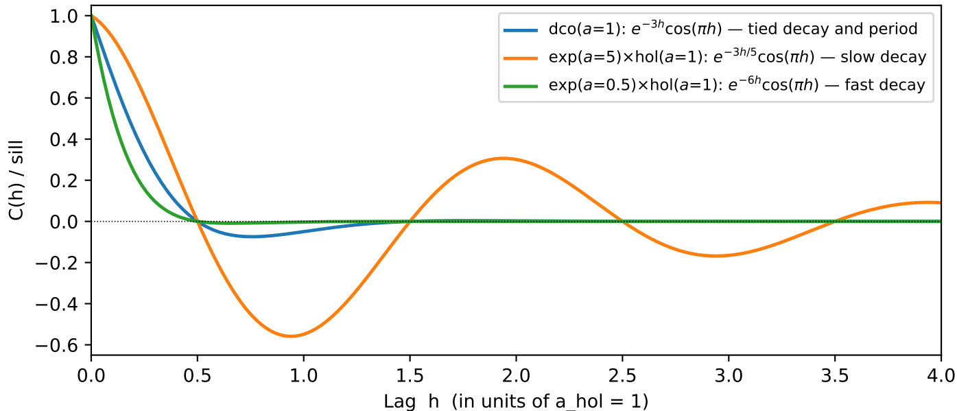
Product variogram: independent a_{\text{exp}} (decay) and a_{\text{hol}} (period)
